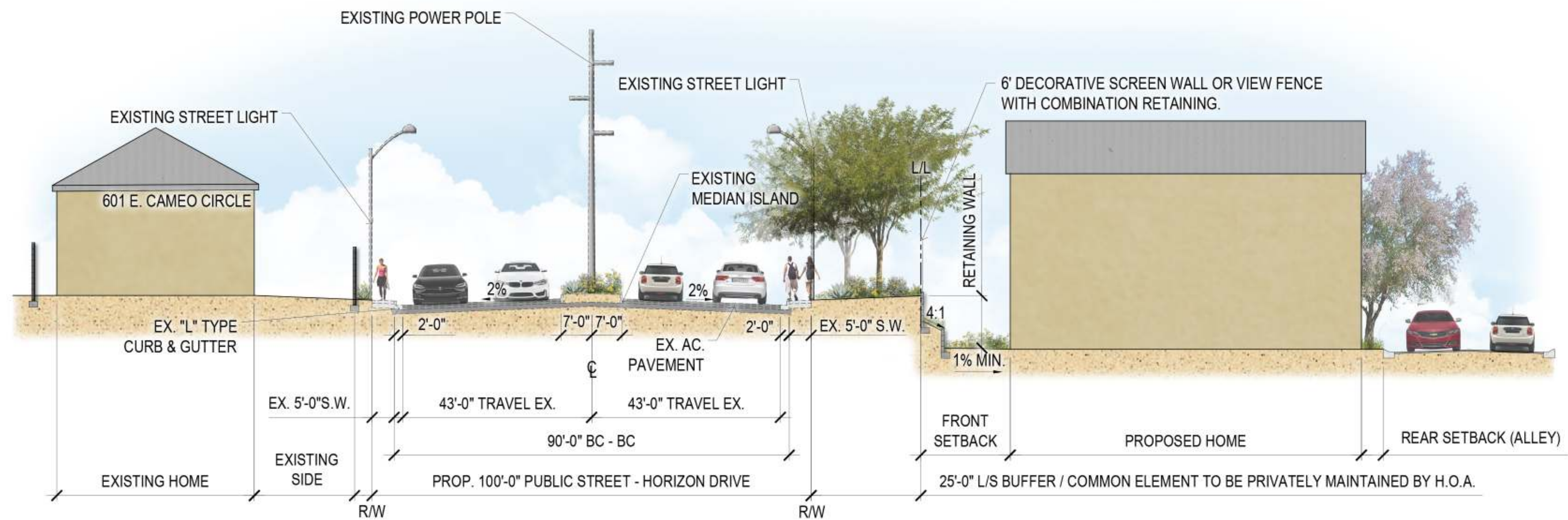
SECTION 19 - HORIZON DRIVE MAXIMUM SLOPE CONDITION (LOOKING WEST)
