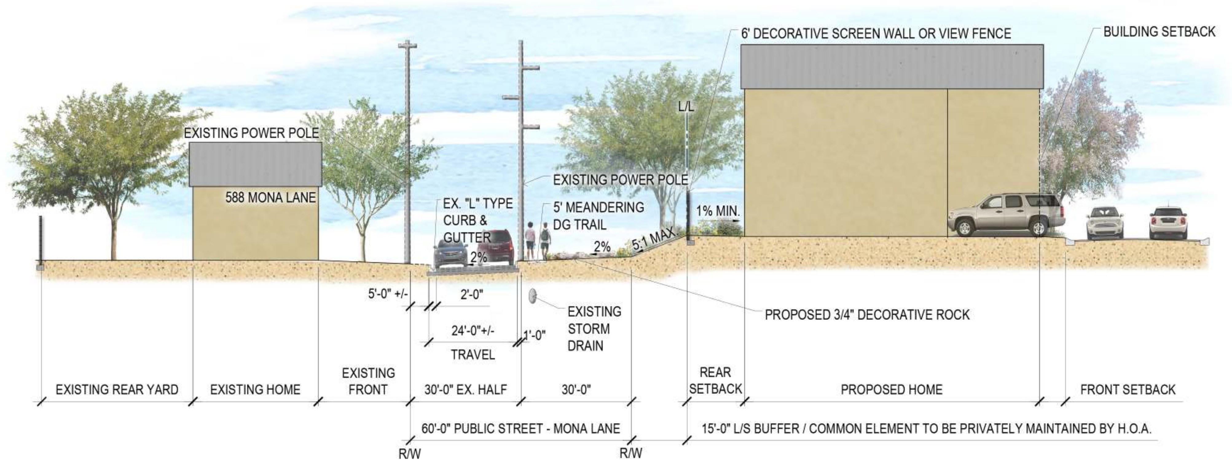
SECTION 17 - MONA LANE MAXIMUM SLOPE CONDITION (LOOKING SOUTH)
