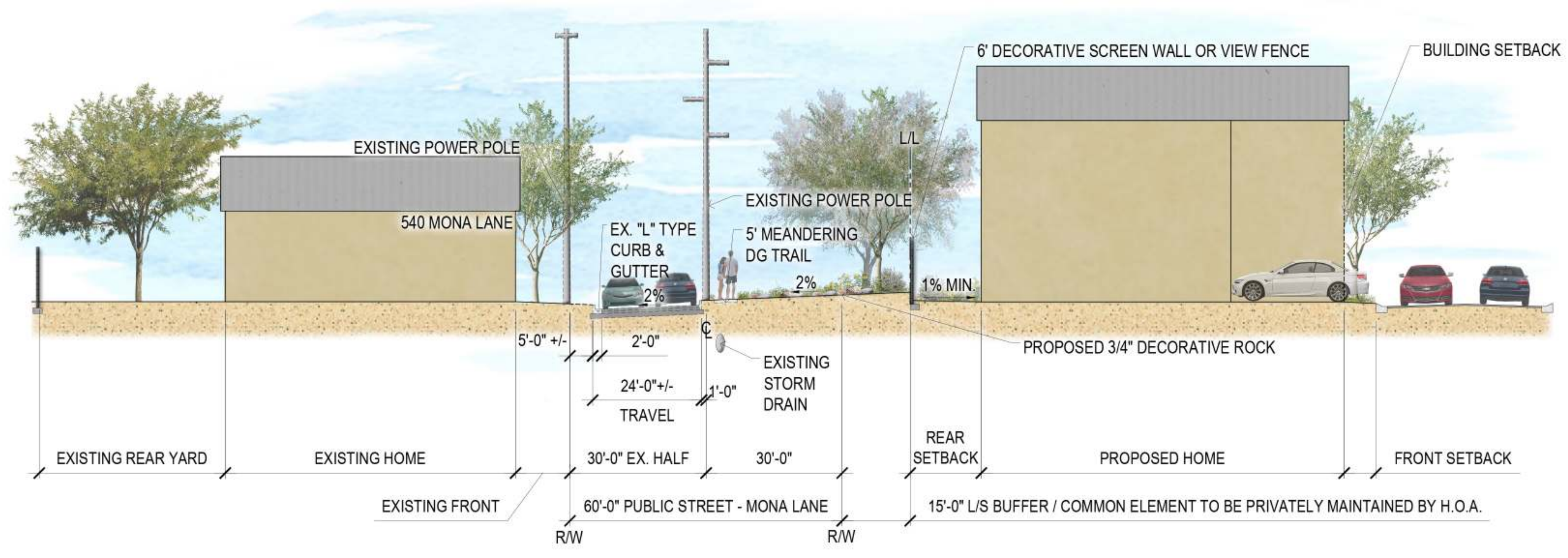
SECTION 16 - MONA LANE MINIMUM SLOPE CONDITION (LOOKING SOUTH)
