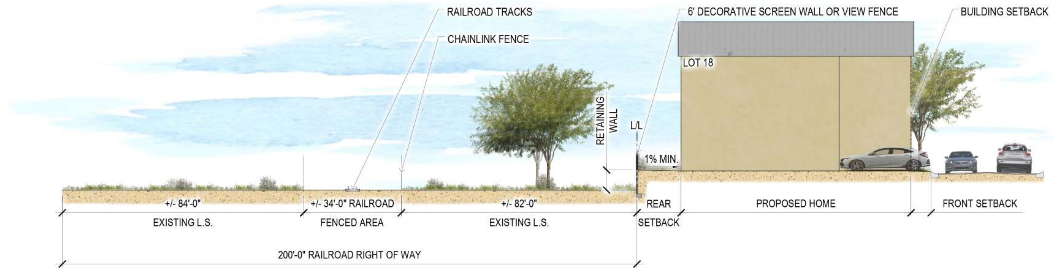
SECTION 14 - UNION PACIFIC RAILROAD MINIMUM SLOPE CONDITION (LOOKING NORTHEAST)
