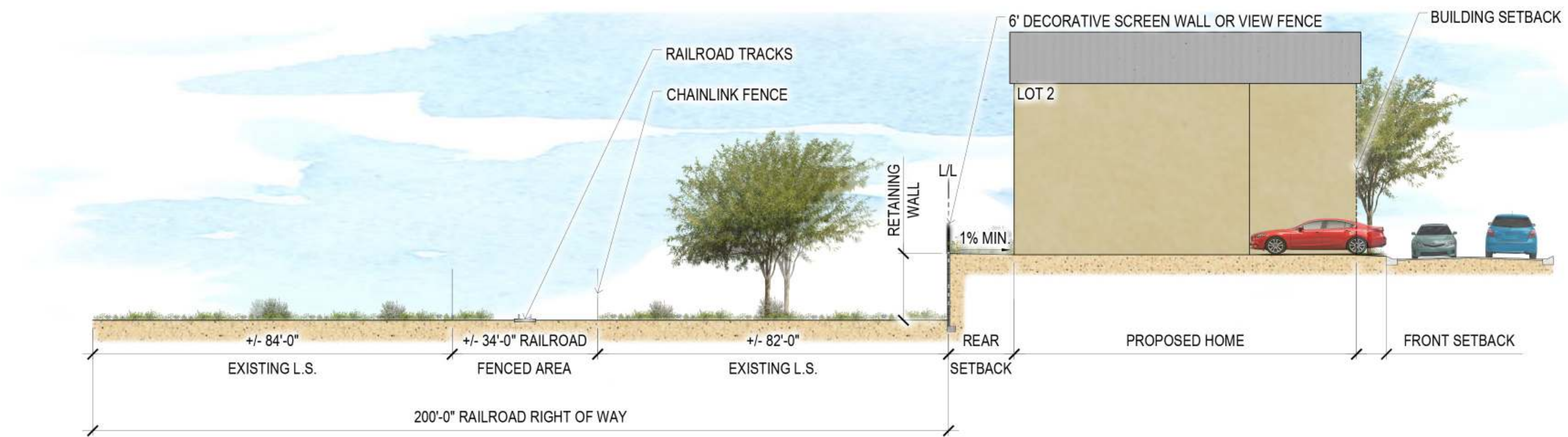
SECTION 15 - UNION PACIFIC RAILROAD MAXIMUM SLOPE CONDITION (LOOKING NORTHEAST)
