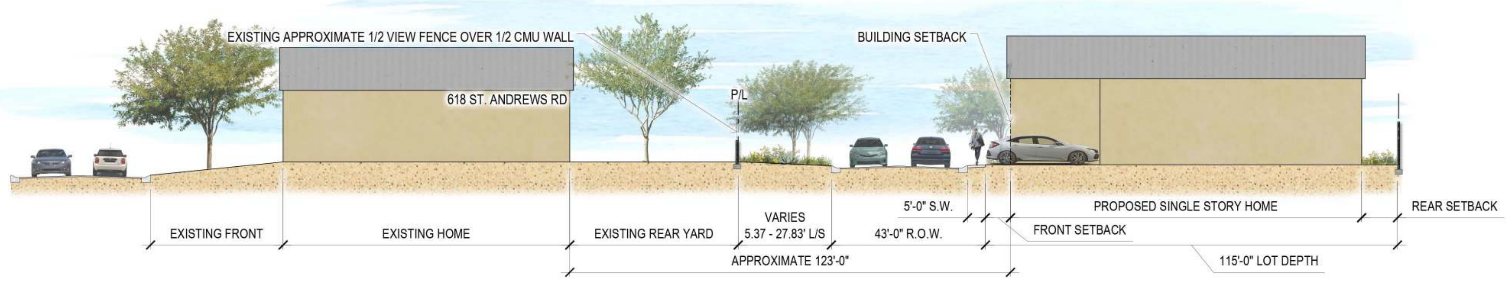
SECTION 1 - 618 ST ANDREWS ROAD (LOOKING NORTH)
