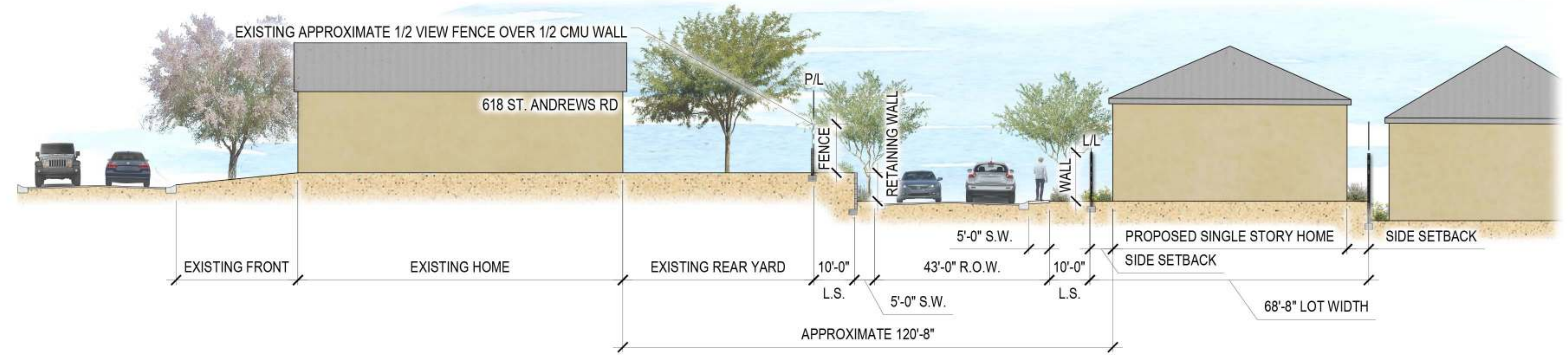
SECTION 2 - 618 ST ANDREWS ROAD (LOOKING SOUTHWEST)
